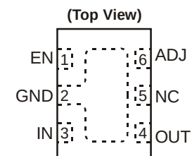
U-DFN2020-6 (ADJ Output) (SN Package)
