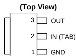
SOT223 (Fixed output) (ER Package)
