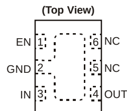
U-DFN2020-6 (Fixed Output) (SN Package)
