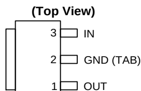
SOT223 (Fixed output) (E Package)
